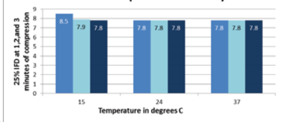
CoolFlow™ Temperature Sensitivity
