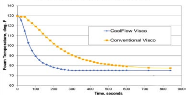
Temperature Transmission Rate Comparison Dynamic Constant Force Air Transmission (0.70 Kpa)
