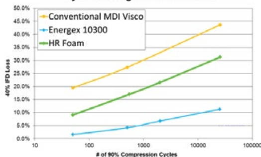
Dynamic Fatigue - 40% IFD Loss
